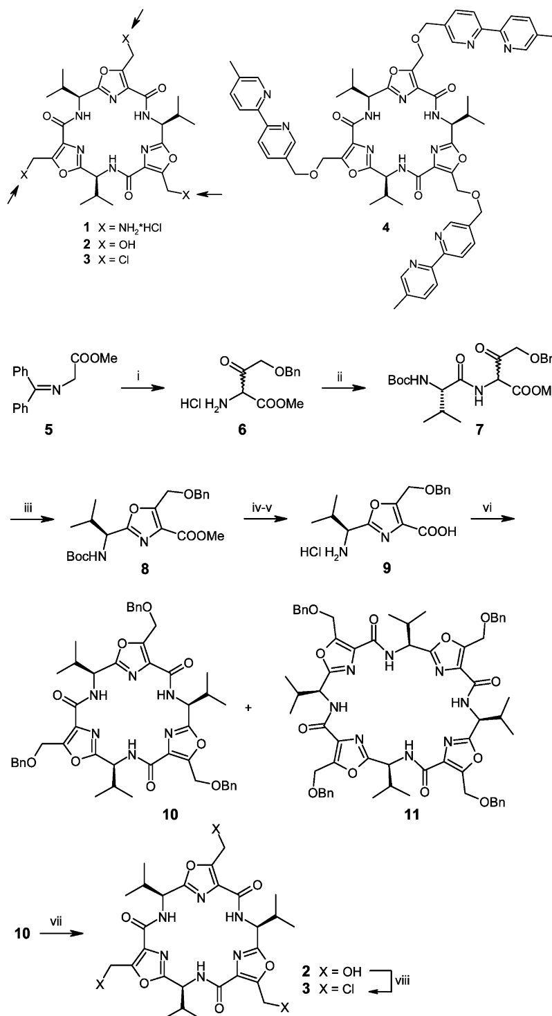
Scheme 1. Synthesis of scaffolds 2 and 3 : i) BnOCH 2 COCl, KO t Bu, THF, then 2 M HCl/H 2 O, -60 °C, 76%. ii) Boc-L-Val-OH, i BuOCOCl, NMM, DCM, -40 °C → r.t., 55%. iii) PPh 3 , Et 3 N, C 2 Cl 6 , DCM, room temp., 71%. iv) 2 M NaOH, MeOH/1,4-dioxane, 97%; v) HCl, EtOAc, 99%; vi) PyBOP, i Pr 2 NEt, DMF, room temp., 39% for 10 and 13% for 11 . vii) Pd/C, H 2 , DCM, 99%. viii) SOCl 2 , CHCl 3 , Δ, 99%.
