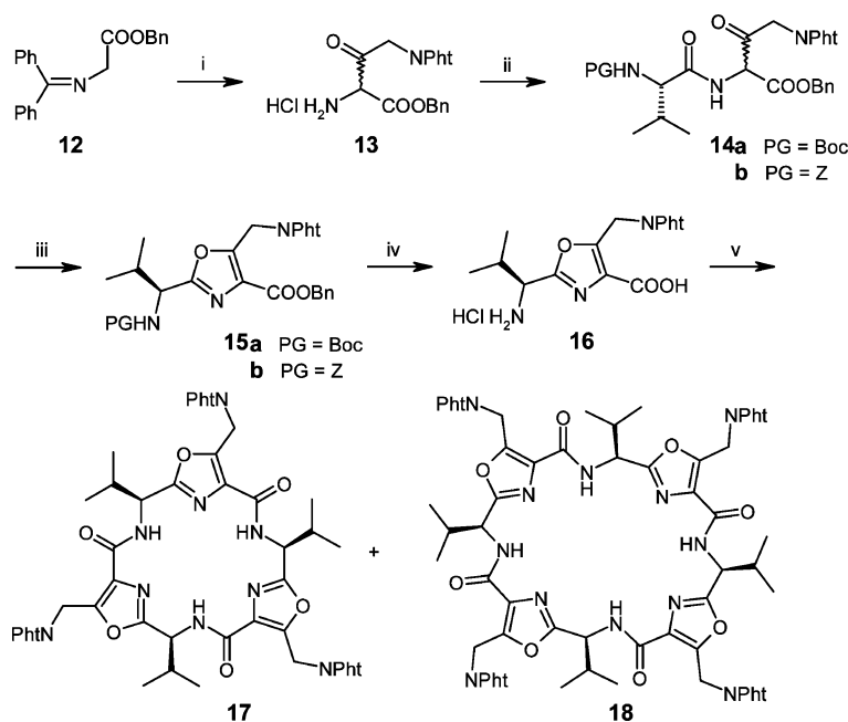
Scheme 2. Synthesis of scaffolds 17 and 18 : i) PhtNCH 2 COCl, KO t Bu, THF, then 2 M HCl/H 2 O, –60 °C, 84%. ii) Boc-L-Val-OH or Z -L-Val-OH, i BuOCOC1, NMM, THF or DCM, –25 °C → r.t., 65% for 14a and 88% for 14b . iii) PPh 3 , Et 3 N, C 2 Cl 6 , DCM, room temp., 52% for 15a and 76% for 15b . (iv) 15a : Pd(OH) 2 /C, H 2 , MeOH, 98% and HCl, EtOAc, 98%; 15b : Pd(OH) 2 /C, H 2 , aq. HCl, MeOH, 99%; (v) PyBOP, i Pr 2 NEt, DMF, room temp., 32% for 17 and 11% for 18 .
