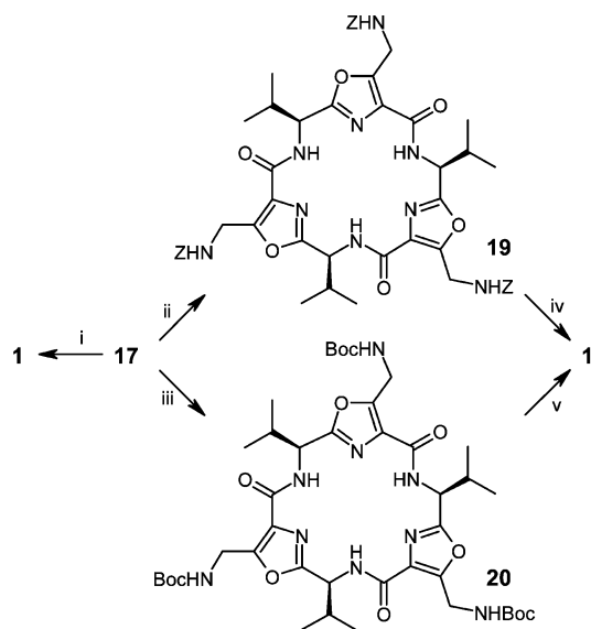
Scheme 3. Synthesis of scaffold 1 : i) NH 2 NH 2 ·H 2 O, THF/DCM/EtOH, r.t. then acidic work-up, 81%. ii) 1. NH 2 NH 2 ·H 2 O, THF/DCM/EtOH, room temp., 2. Z-Cl, Et 3 N, DCM, room temp., 57%. iii) NH 2 NH 2 ·H 2 O, THF/DCM/EtOH then Boc 2 O, room temp., 92%. iv) Pd/C, H 2 , aq. HCl, MeOH, room temp., 88%. v) HCl, EtOAc, room temp., 100%.
