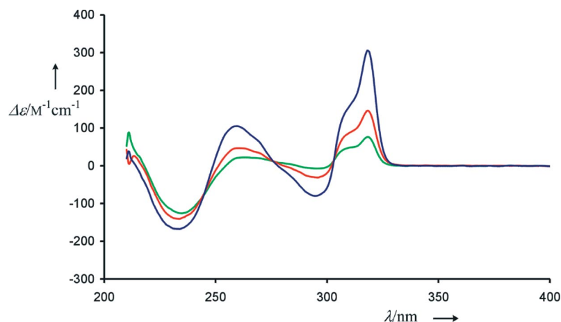
Figure 1. CD spectra of the ligand 4 (green) with \text{CuCl}_2 (red) and \text{ZnCl}_2 (blue) in \text{MeOH}/\text{H}_2\text{O} (1:1; buffer: 0.10 M TRIS, 0.02 M HCl in \text{H}_2\text{O} ) ( [\mathbf{4}] = 1.6 \times 10^{-5} \text{ M} and \mathbf{4}/\text{M}^{2+} = 1:1 ).
