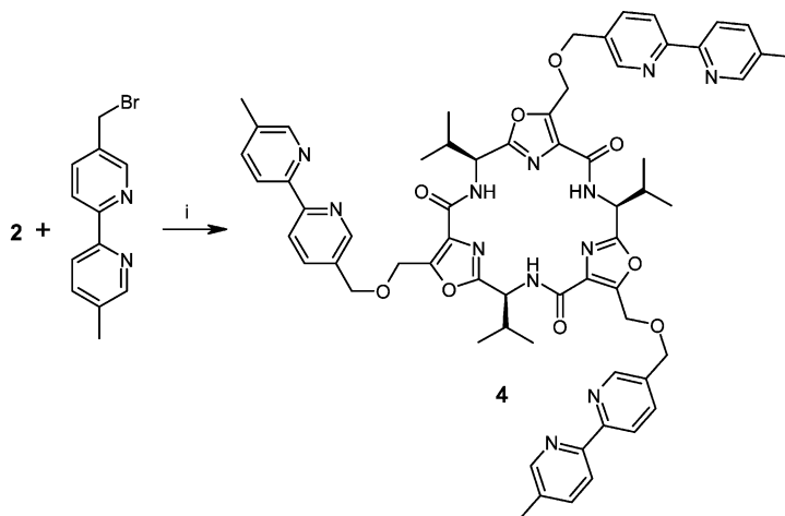
Scheme 4. Synthesis of ligand 4 : i) NaH, THF, r.t. → 4 , 33%.
