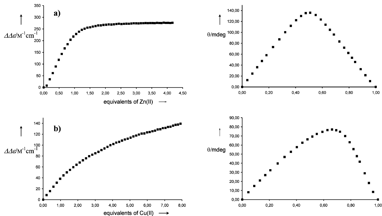
Figure 2. Plot of \Delta\Delta\epsilon vs. equivalents of metal ions and Job-plots \{y = \theta_{\text{obs}} - \theta_{\text{L}} - (\theta_{\text{M}} - \theta_{\text{L}}) \cdot x \text{ vs. } x = [\text{M}]/([\text{M}] + [\text{L}])\} for complexation of 4 with \text{Zn}^{\text{II}} (a) and \text{Cu}^{\text{II}} (b), respectively. The values were recorded at 318 nm.
